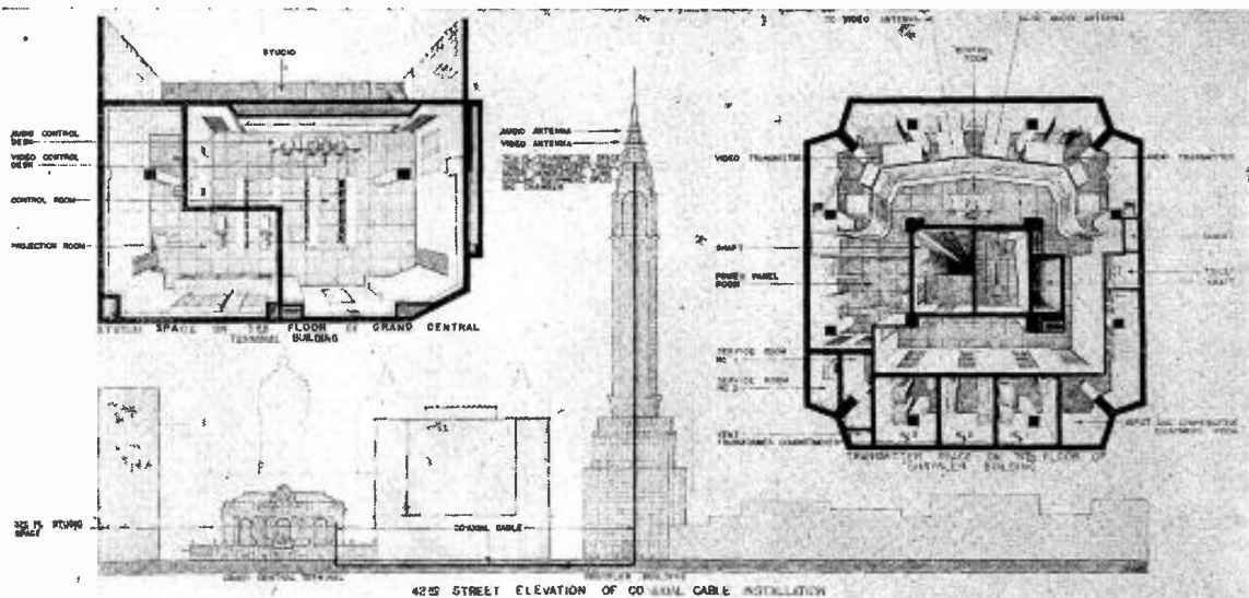
42ND STREET ELEVATION OF COAXIAL CABLE INSTALLATION
